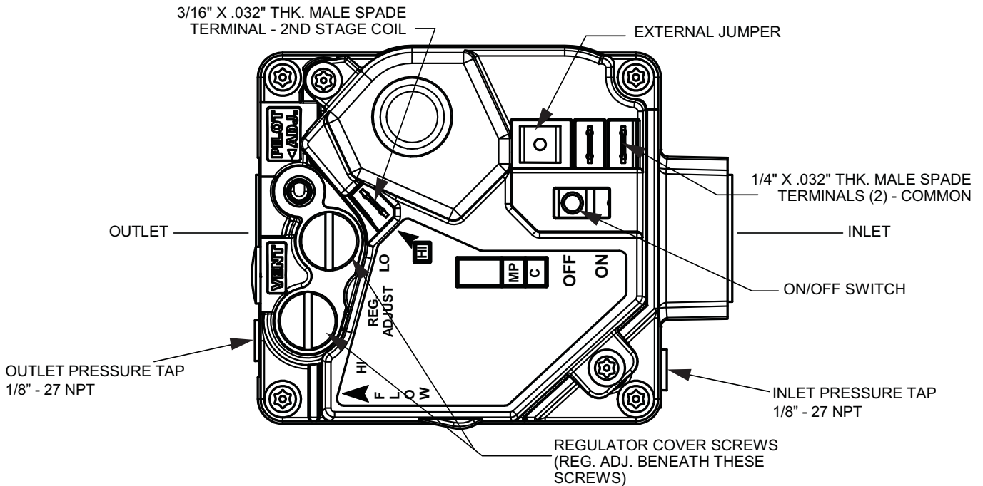
Figure 29: 6 Thru 12.5 Ton 3/4" Two Stage Gas Valve
