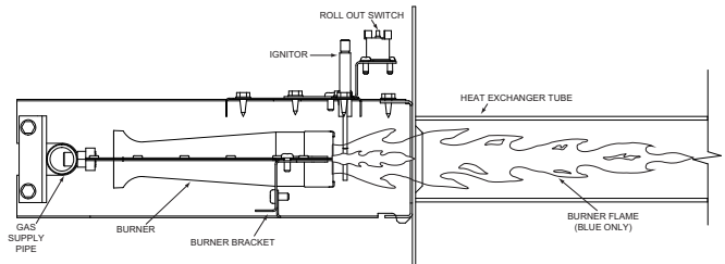
Figure 26: Typical Flame
