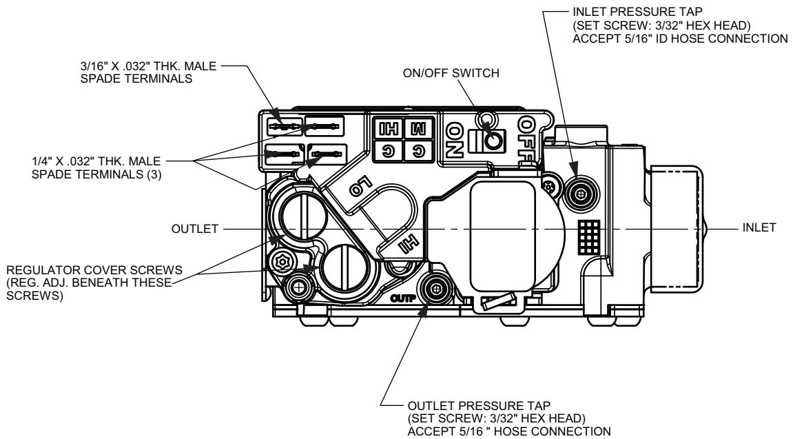
Figure 28: 3 Thru 5 Ton, 1/2" Two Stage Gas Valve
