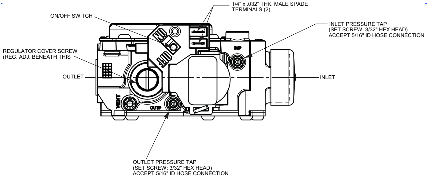
Figure 27: 3 Thru 5 Ton, 1/2" Single Stage Gas Valve
